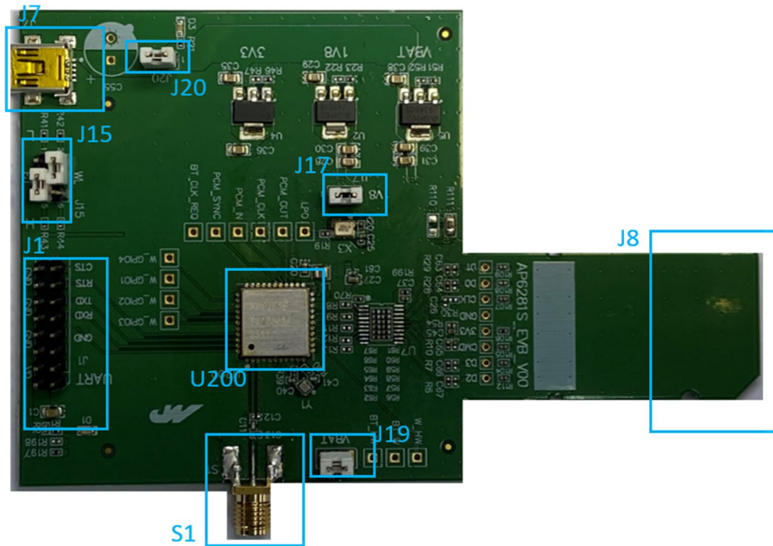
Figure1. Top view of AP6745 EVB
